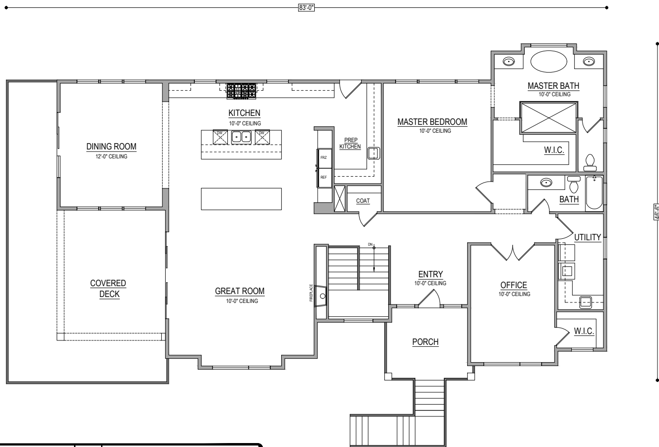
1 MAIN FLOOR PLAN (2587 SF)
